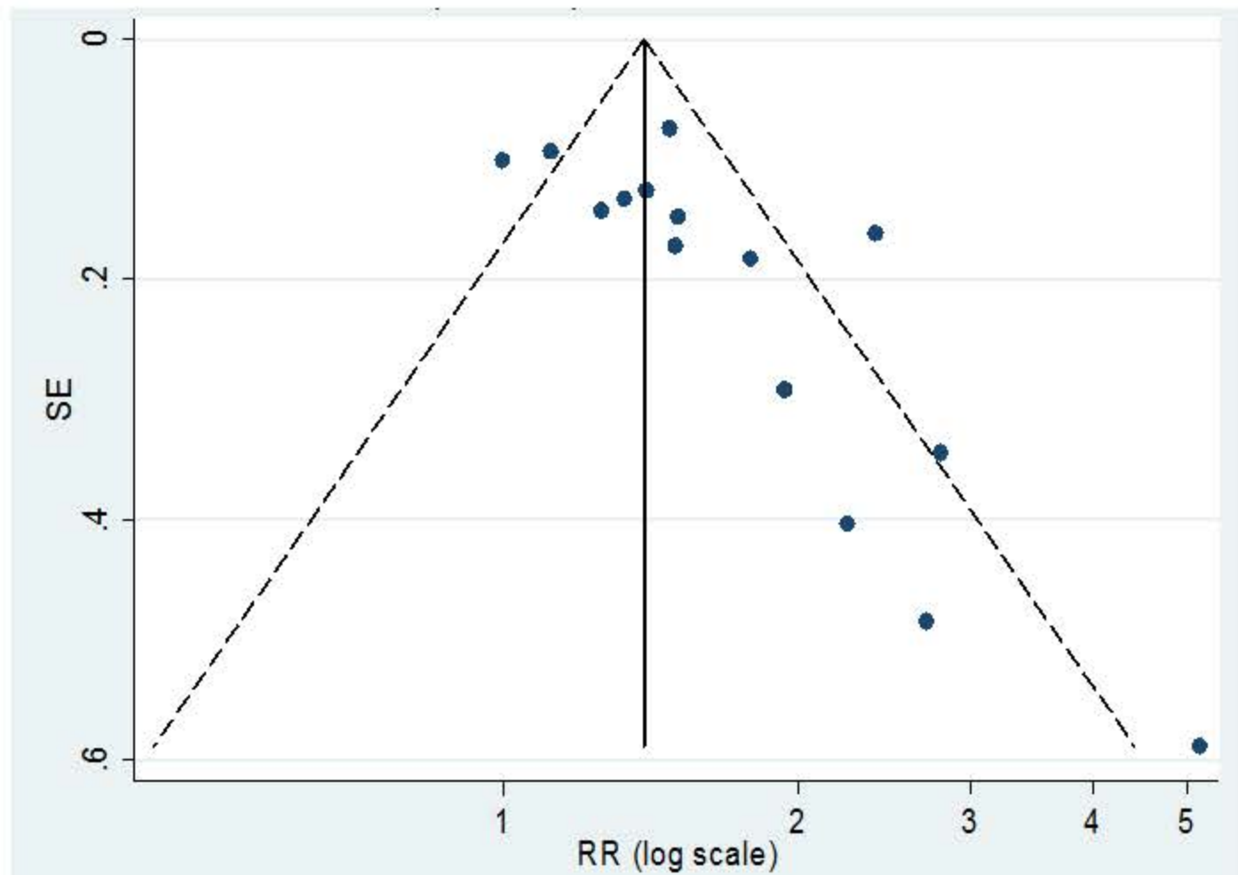
A Funnel plot with pseudo 95% confidence limits
